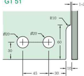
Fin Notching detail GT 51
