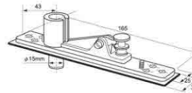
9118 Adjustable top centre
