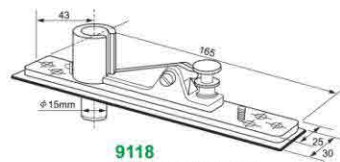
9118 Adjustable top centre
