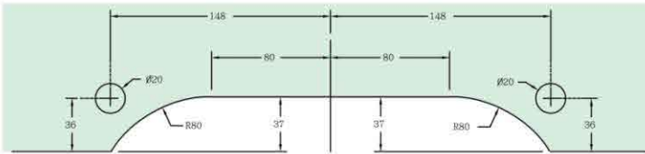
Notching detail GL 50/2K GL 50/2KS GT 51
