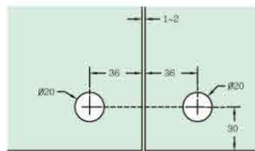
GT 70 Notching detail-double panels
