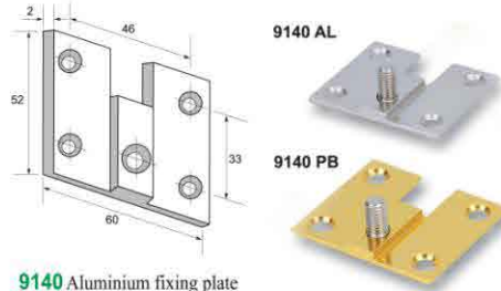
9140 Aluminium fixing plate (Optional for GT30, GT30/K)
