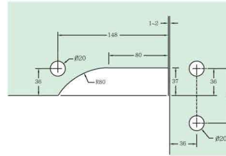
Notching detail GT 40, GT 40/K, GT 40/S, GT 40/KS GT 41, GT 41/K, GT 41/KS
