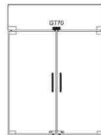
GT 70 Notching detail-double panels
