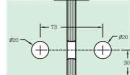
GT 71 FIN Notching detail
