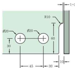
Fin Notching detail GT41, GT41/K, GT41/KS
