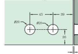
GT 71 FIN Notching detail
